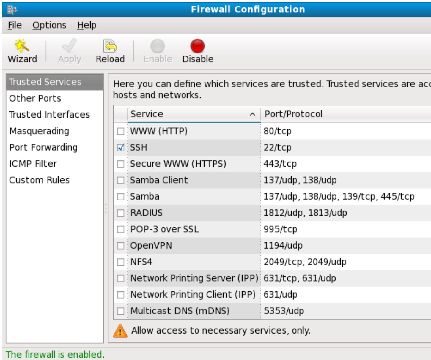
Figure 2.5. Firewall Configuration Tool
